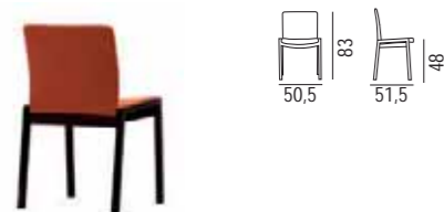
LIVIO | PAG. 090 - 093 Finiture / finishes: TF100, TF101, TF102, TF110, L9017, L9016, L1015, L1018, L1032, L2004, L3014, L3017, L3020, L5012, L5017, L6017, L6019
