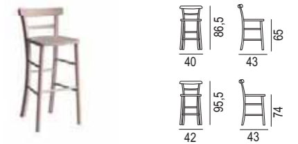
VIOLINIST STOOL | PAG. 158 - 161 Finiture / finishes: TF100, TF101, TF102, TF110, L9017, L9016, L1015, L1018, L1032, L2004, L3014, L3017, L3020, L5012, L5017, L6017, L6019
