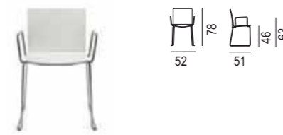
METROPOLIS CHAIR | PAG. 104 - 111 Finiture scocca / shell finishes: PT100, PT111, PT112, PT114 Finiture base / frame finishes: MC100, M9017, M9016 Scocca in tecnopolimero o imbottita. Tecnopolymer or upholstered shell.
