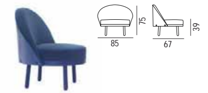
METROPOLIS CHAIR | PAG. 104 - 111 Finiture base / frame finishes: MC100, M9017, M9016 Base a slitta o a quattro gambe. Sled or four leg frame.
